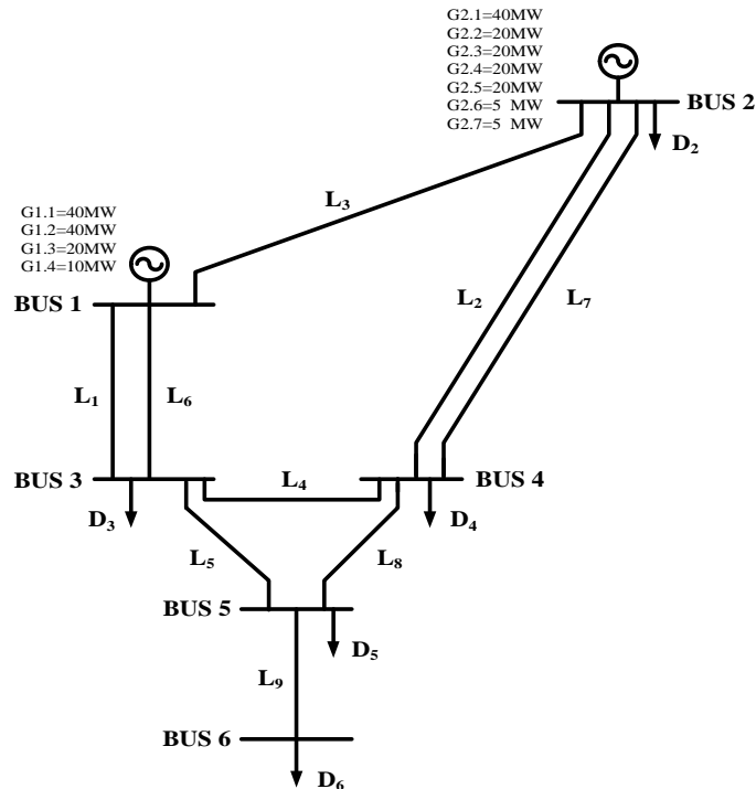
Figure 1. Single-line diagram of RBTS [14]
