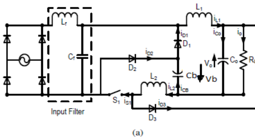
Figure 1. Proposed Integrated Buck Buck-Boost Converter
