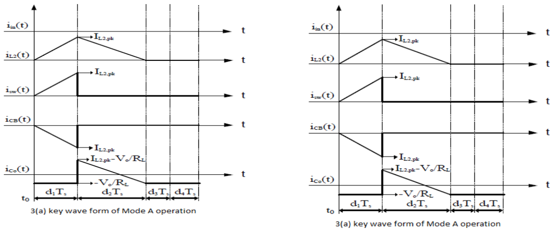
Figure 3. Key wave form of Mode A operation
