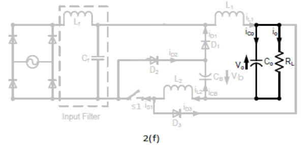
Figure 2. Circuit representation the corresponding proposed buck buck-boost converter.
